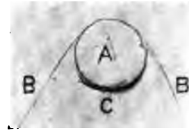
FIG. 118A. A is a section of the Egret. B the roof-like plumes. C the dark underside which they hide. The part of a heron's neck that normally bends backward as he stands has the roof's ridge-pole in front, and the eaves behind.
